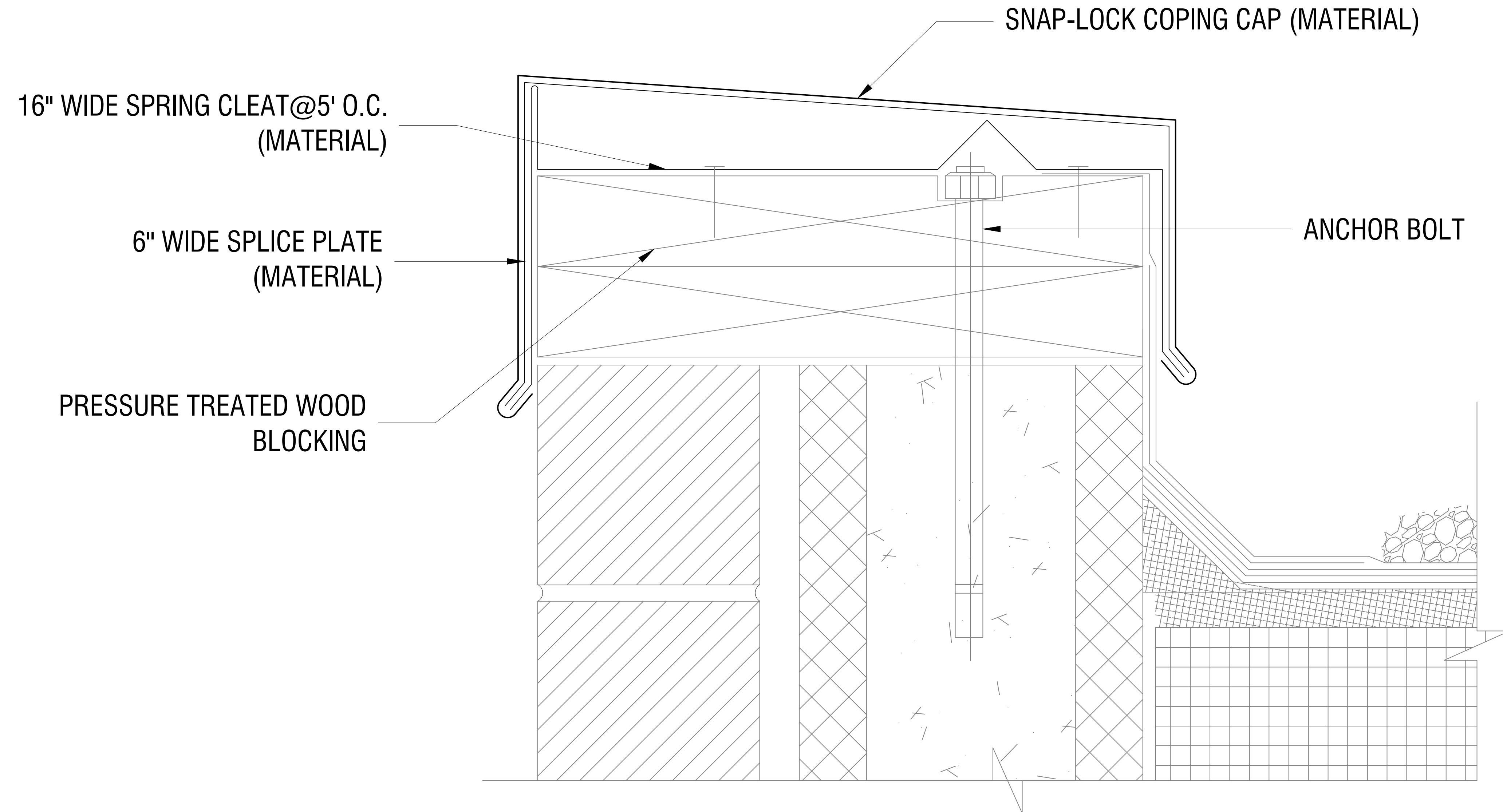
1 TYPICAL SECTION DETAIL AT COPING SCALE: NTS.
