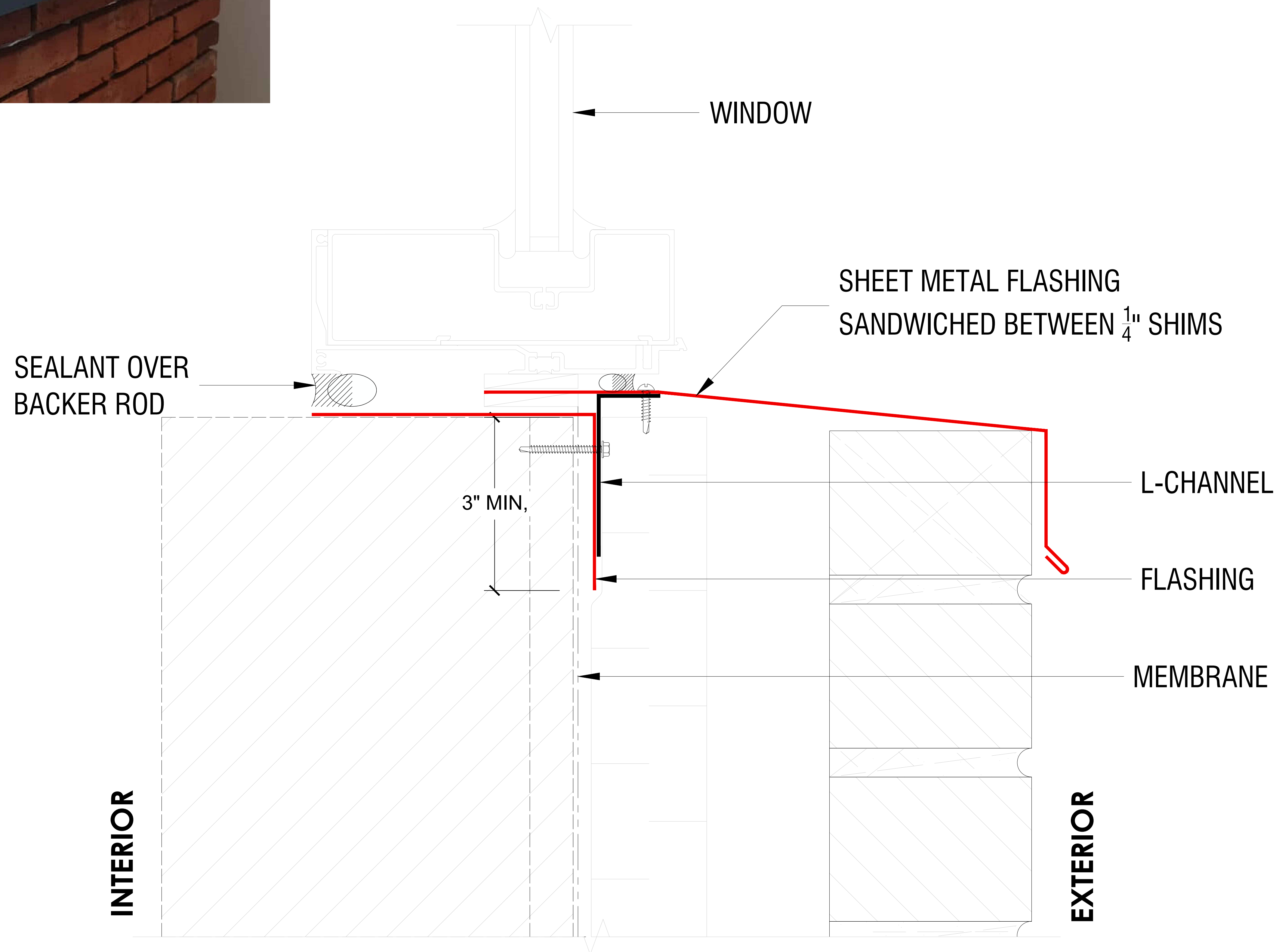
1 WINDOW SILL DETAIL SCALE: NTS.
